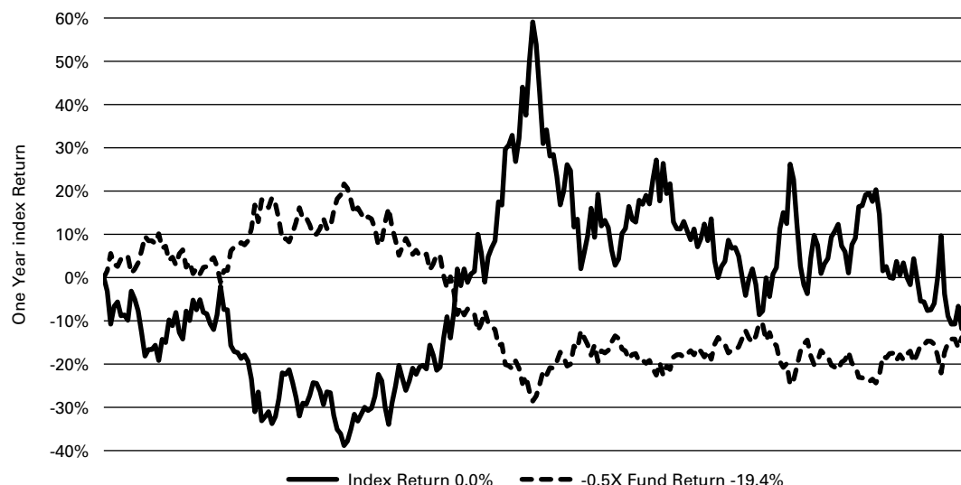
One-Year Simulation; Benchmark Flat (0%) (Annualized Benchmark Volatility 76%)
