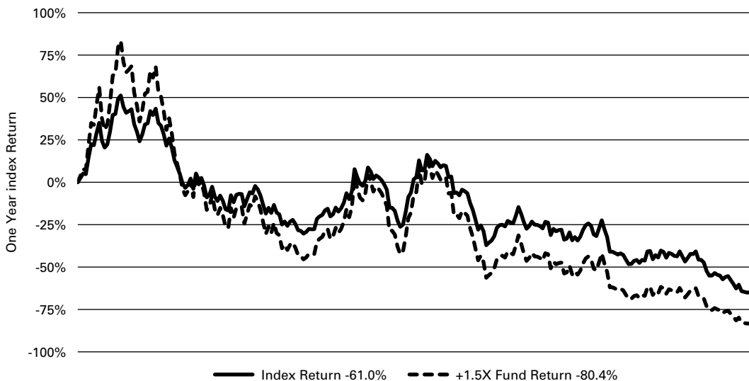
One-Year Simulation; Benchmark Down 61% (Annualized Benchmark Volatility 76%)
