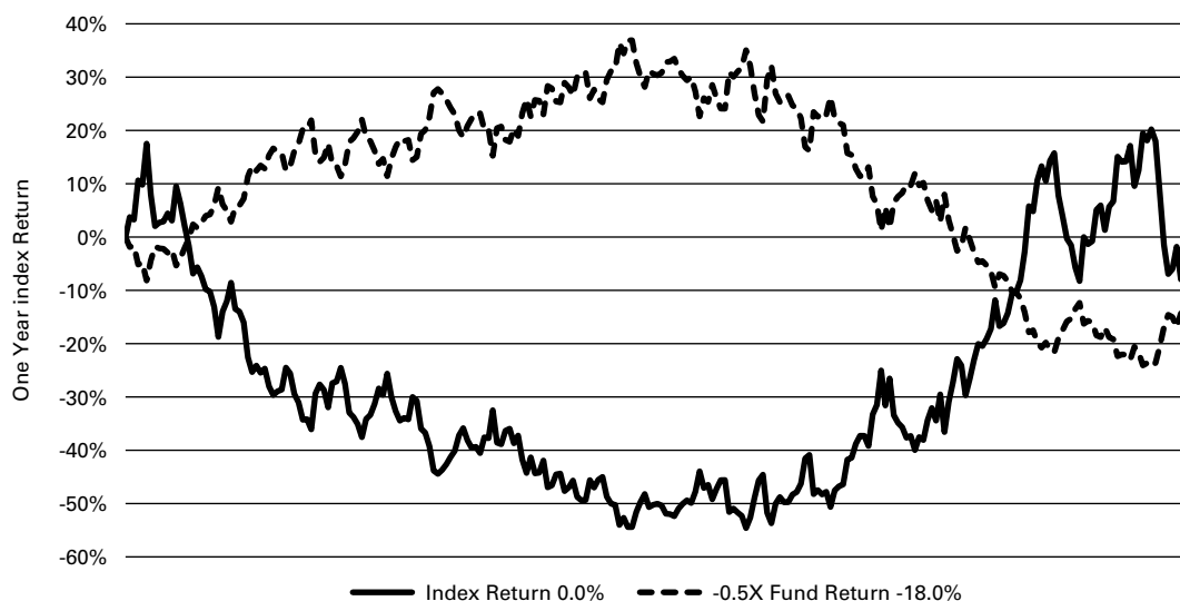
One-Year Simulation; Benchmark Flat (0%) (Annualized Benchmark Volatility 73%)
